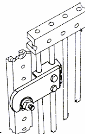
B-RF Bayonet (in line) 'R' panel to 'F' panel.
