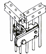
AB-RR Angle - Bayonet — 'R' panel to 'R' panel.
