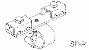
SP-R Side Plate Connector Tube to Rods
