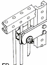
B-FR Bayonet (in line) 'F' panel to 'R' panel.
