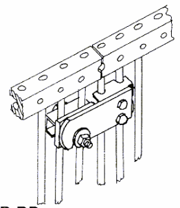
B-RR Bayonet (in line) 'R' panel to 'R' panel.
