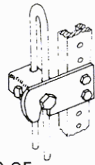
AB-CF Angle - Bayonet — 'C' panel to 'F' panel.
