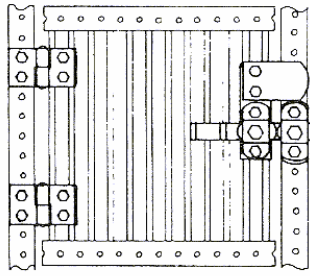
H-FR Hinged Panel 'R' panel to 'F' const.
