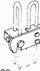
AB-CC Angle - Bayonet 'C' panel to 'C' panel.
