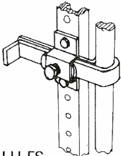
LH-FS Hook Latch Conn. 'F' panel to stud
