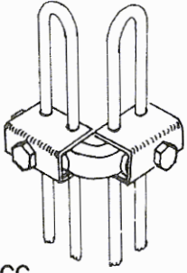
A-CC Angle — 'C' panel to 'C' panel.
